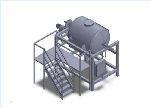
蒸煮設備 Steaming Equipment
